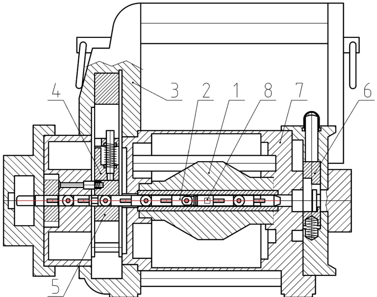
Picture 1 Radiation heads of gamma-projectors RID-Se4UM P (Exertus Light) and RID-Se4WM P (Exertus Light W)
