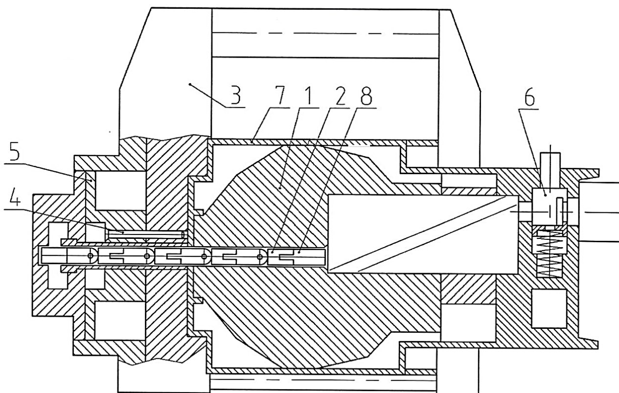
Radiation head of gamma-projector "Exertus Dual 120"
