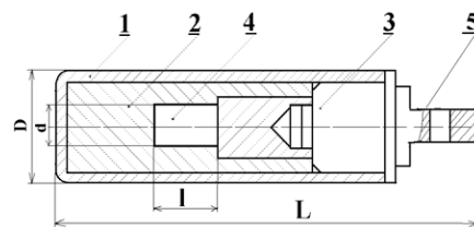
c) GS75M13 (the capsule has a blade-shaped tail)
