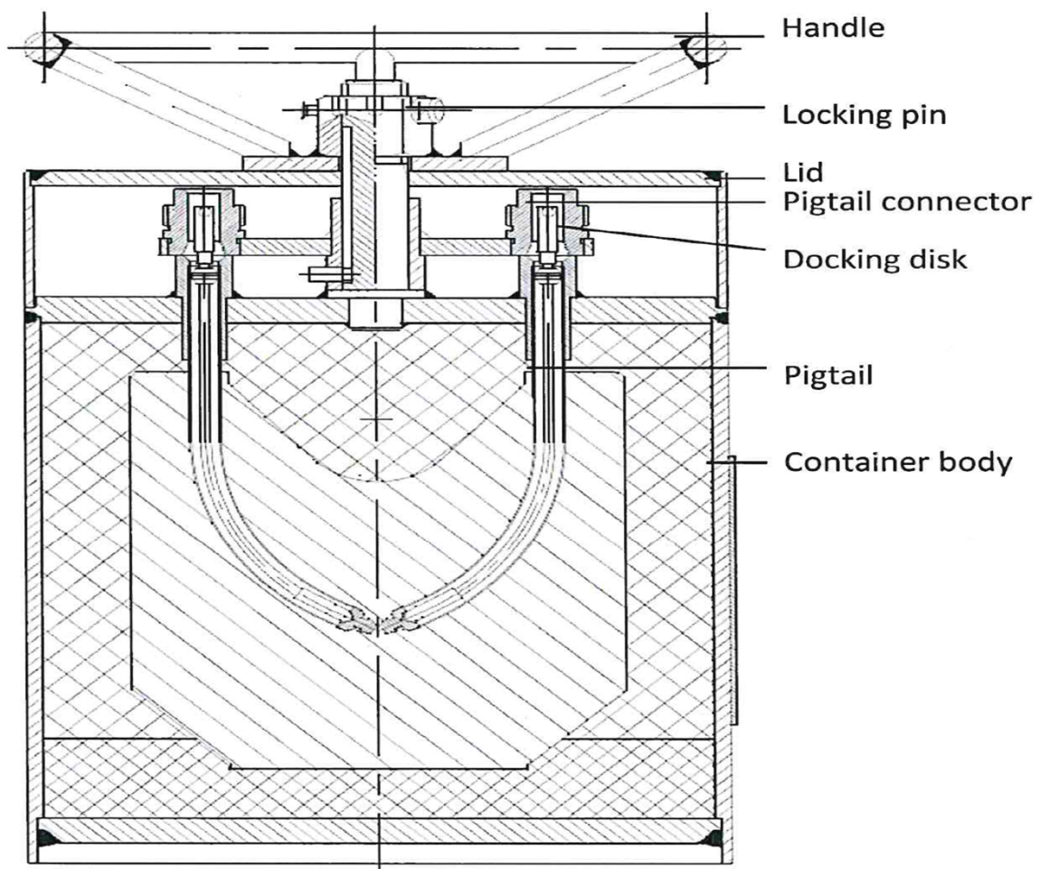
Figure 1: Outline Drawing of Transport Package: ZA ZA/NNR 1004/B(U)-96
