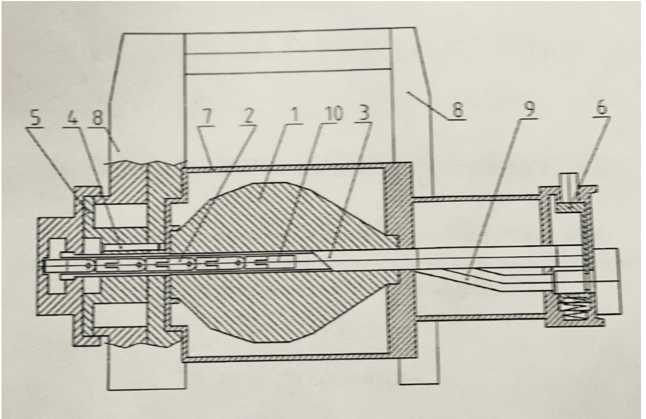
Picture 1 Radiation head of gamma-projector RID-Se-Ir/60 (Exertus Novum)
