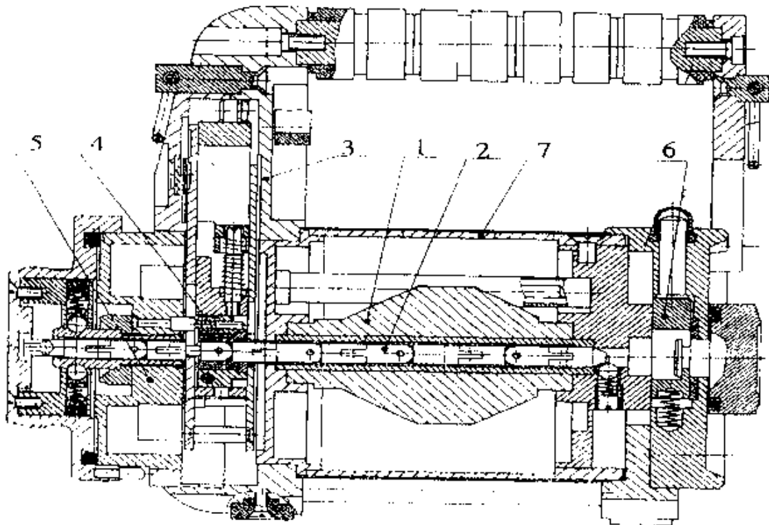
Picture 1. Radiation head of gamma-defectoscope RID-Se4UM P (Exertus Light)
